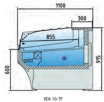
VEA-10-TF
