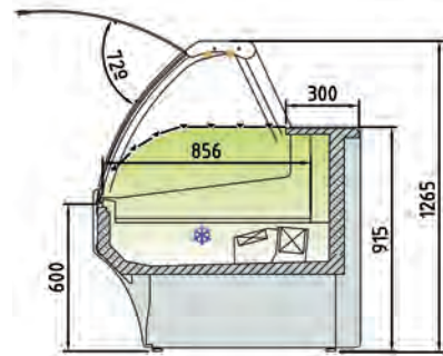
VES-10E-C-TF
