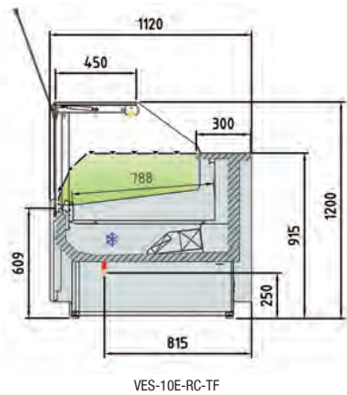
VES-10E-RC-TF
