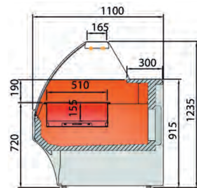
VE-10-RR HE
