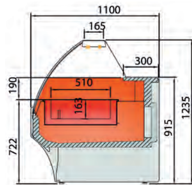
VE-10-RR BM
