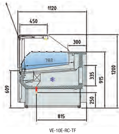
VE-10E-RC-TF
